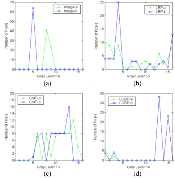
Figure 3. Robustness of the different histograms to images with lighting variation.
