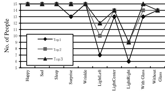
Figure 4 Experiments of the Yale face database
